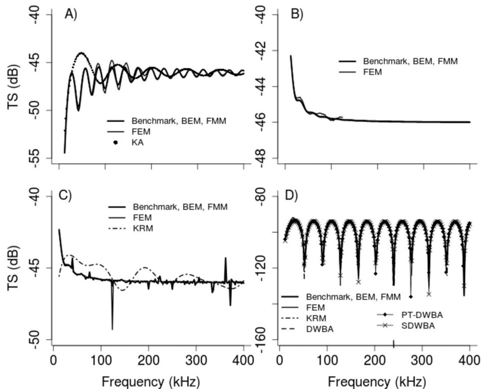
FIG. 3. TS (dB re 1 m 2 ) as a function of frequency ( f ; kHz) for a 0.01-m-radius homogeneous sphere with (A) rigid, (B) pressure-release, (C) gas-filled, and (D) weakly scattering boundary conditions as predicted by the benchmark, BEM, FMM, FEM, KA, KRM, DWBA, PT-DWBA, and SDWBA models. In (A), (B), and (D), TS predictions coincide for the benchmark, BEM, and FMM models. Not all models predicted TS over the full frequency range (Table III).
