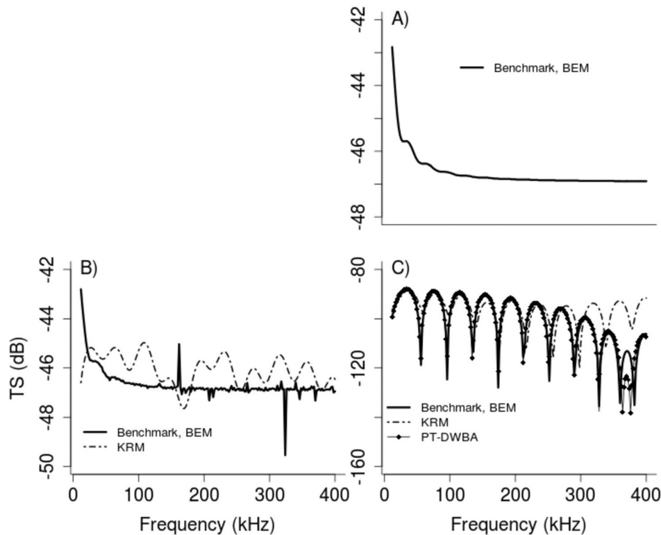
FIG. 4. TS (dB re 1 m 2 ) as a function of frequency ( f ; kHz) for a 0.01-m-radius spherical fluid shell target with (A) pressure-release, (B) gas-filled, and (C) weakly scattering interior as predicted by the benchmark, BEM, FEM, KRM, and PT-DWBA models. In (A), (B), and (C), TS predictions coincide for the benchmark and BEM models. Not all models predicted TS over the full frequency range (Table III).
